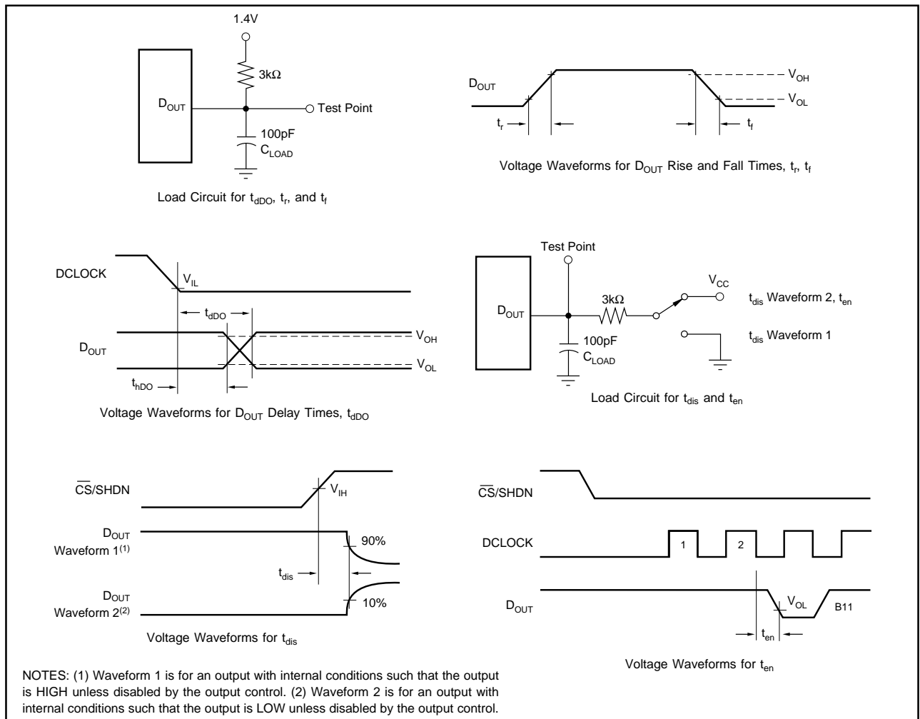
FIGURE 2. Timing Diagrams and Test Circuits for the Parameters in Table I.
